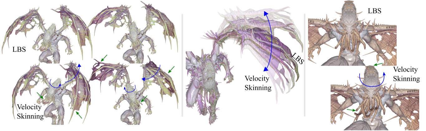
Figure 11: Velocity skinning applied on a detailed mesh, thanks to our GPU implementation. The blue arrows indicates the main motions, while the green arrows highlight some noticeable effects of our deformer. Left: Comparison of LBS (top) and velocity skinning (bottom) on two extreme poses when constant floppy weights are used. Velocity skinning automatically enhances the motion in bending the wings and the tentacles based on their respective bones motion. Middle: Shape variations of the wing applied by the floppy deformer, the "neutral"-LBS pose being the middle one. Right: Computing automatic per-vertex weights based on local shape diameter allows to apply more deformation on mesh details, thus mimicking a lower stiffness on small protruding elements.
